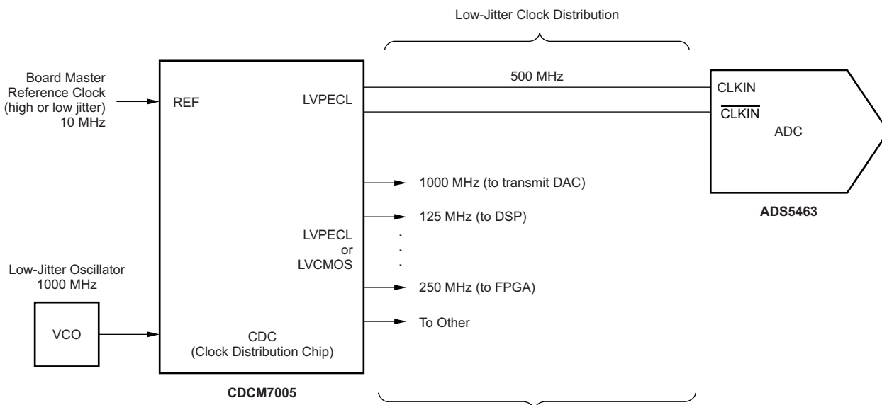
Figure 46. Optimum Jitter Clock Circuit
